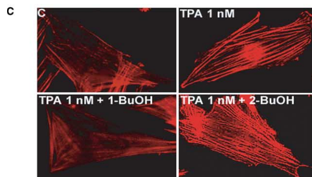
Fig. 5. 1-Butanol selectively inhibits the myogenic response to 1 nM TPA. (A) Cells were cultured in 1% BSA medium, without addition (control), or in the presence of 1 nM TPA, with or without 0.5% 1-butanol or 2-butanol. After 48 h, myogenin immunofluorescence was assessed. (B) The means \pm S.E. of the percentages of myogenin positive nuclei counted in 10 fields were calculated. (C) Actin fibers were stained with rhodamine-phalloidin in cells kept for 15 min without addition (control), or in the presence of 1 nM TPA, with or without 0.5% 1-butanol or 2-butanol.
